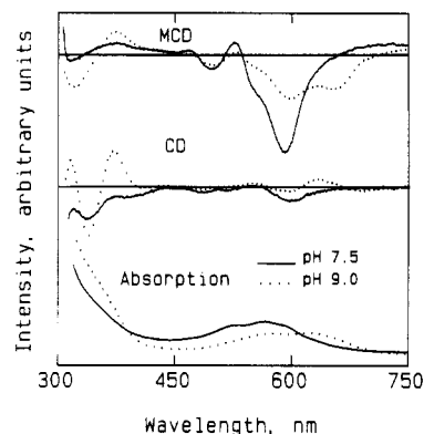
Figure 2. Room-temperature absorption, CD, and MCD spectra of CoHcy at pH 7.5 and pH 9.0. The spectra at pH 7.5 are representative of aquoCoHcy, and the spectra at pH 9.0 are due mostly to hydroxoCoHcy.
